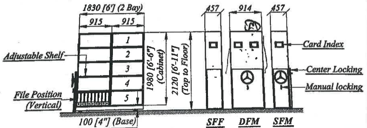
Cabinet Front View
